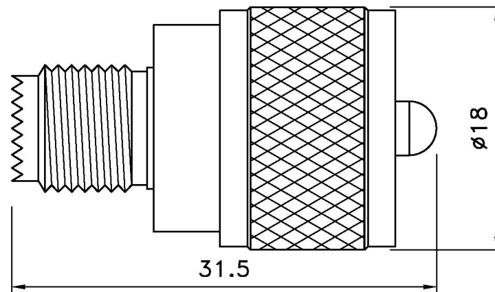
MINI UHF FEMALE TO UHF MALE
