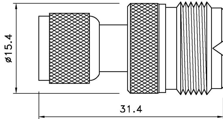
MINI UHF MALE TO UHF FEMALE
